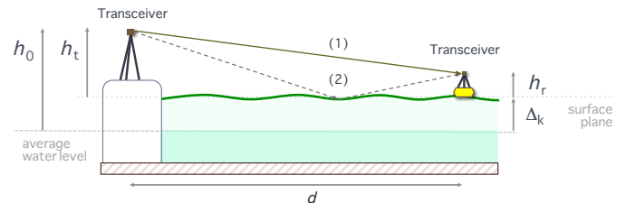
Fig. 1: The two-ray model showing: (1) the direct LoS ray, and (2) the indirect ray reflected from the surface when experiencing a water level variation of \Delta_k .
