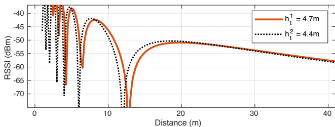
Fig. 2: Received Signal Strength (RSS) as a function of the distance to shore in the near-shore region, for two moments in the tide, leading to two slightly different antenna heights.
