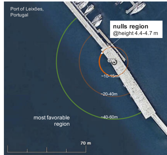
Fig. 6: Top view of the quay in the harbor showing favorable (solid green), transition (brown) and unfavorable (red) regions for the shore-to-AUV WiFi link.
